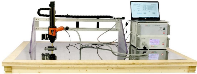
ES614-500 ESD Air Discharge Workstation
